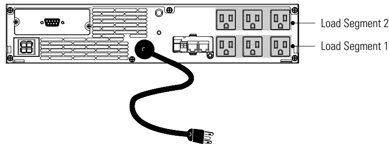
Figure 19. UPS Load Segments (Low Voltage Models)
