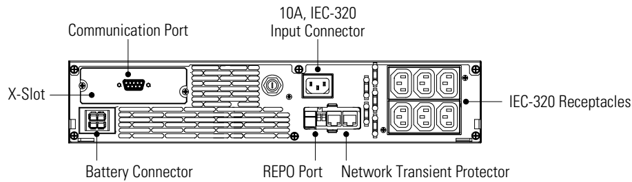
Figure 11. 1000/1500 VA, 230V Rear Panel
