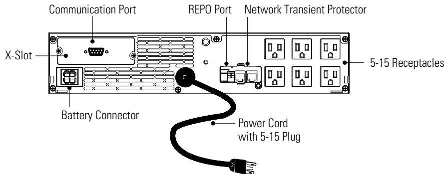
Figure 10. 1000/1500 VA, 120V and 1000 VA, 100V Rear Panel
