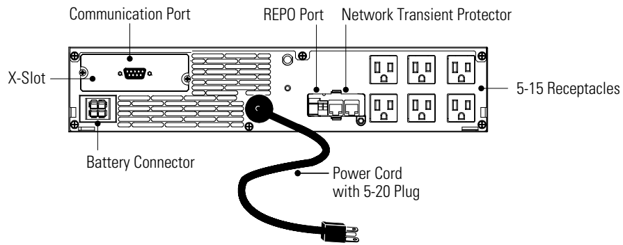
Figure 12. 1500 VA, 100V Rear Panel
