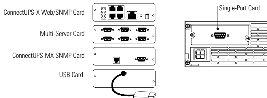
Figure 16. Optional X-Slot Cards
