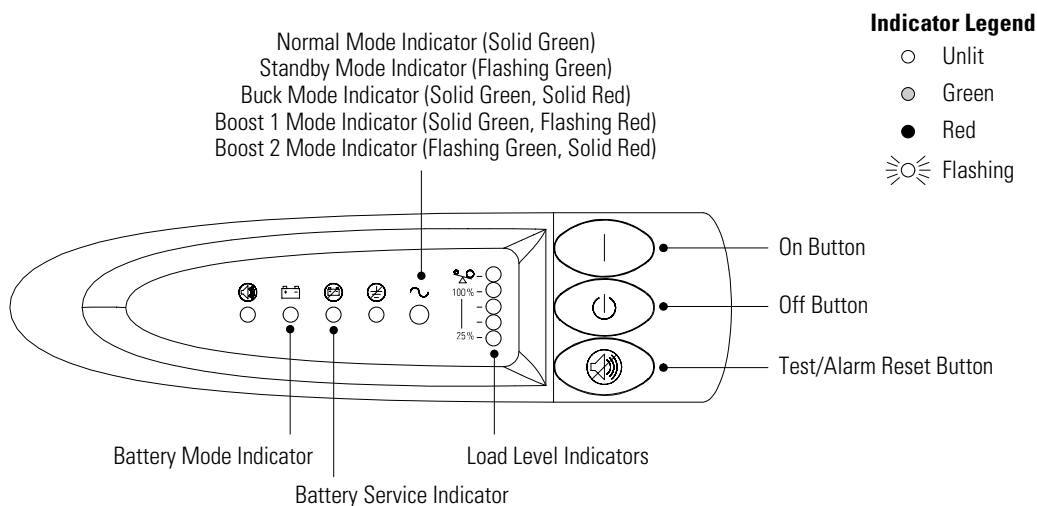
Figure 13. UPS Front Panel
